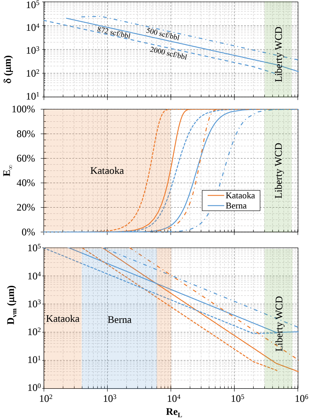
Fig. 2-Plotted \delta , E_\infty , and D_{vm} for a range of Re_L , for 500, 872, and 2000 scf/bbl (51, 155, and 356 \text{m}^3_{\text{gas}}/\text{m}^3_{\text{oil}} ), with the first 90 days of Liberty WCD highlighted green. The validated range of the Kataoka et al. correlation shown highlighted orange and the validated range of Berna et al. is highlighted blue.
