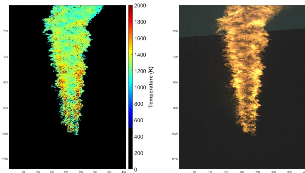
Fig. 51-3g/s of gas ( \text{CH}_4:\text{C}_2\text{H}_6:\text{C}_3\text{H}_8 = 80:5:15 ) and 32g/s of Endicott Crude oil.
