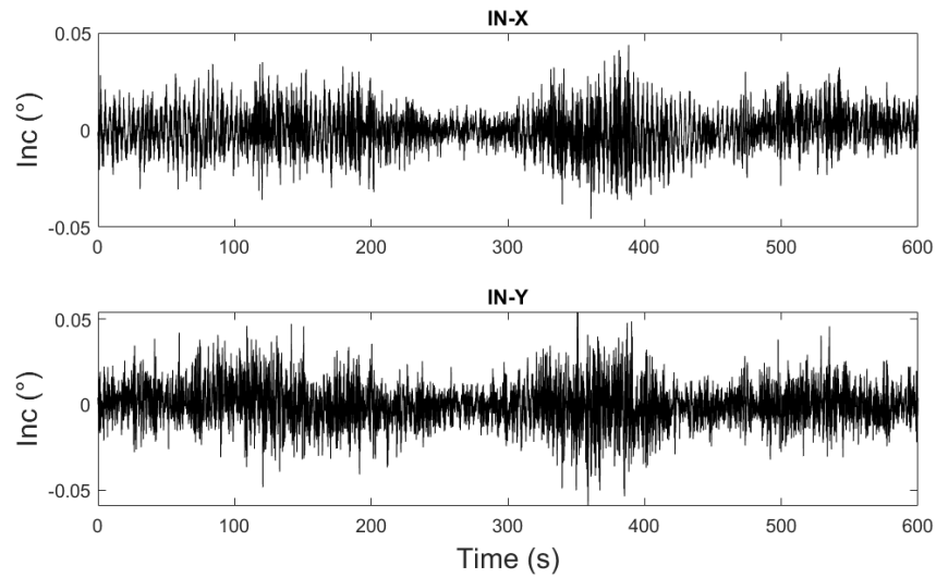
Figure 5. Sample of inclination time histories at 9:17 on April 22.
