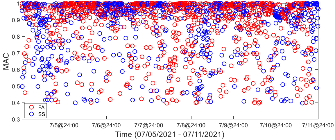
Figure 63. MAC evolution of identified FA/SS modes from 7/5 to 7/11.
