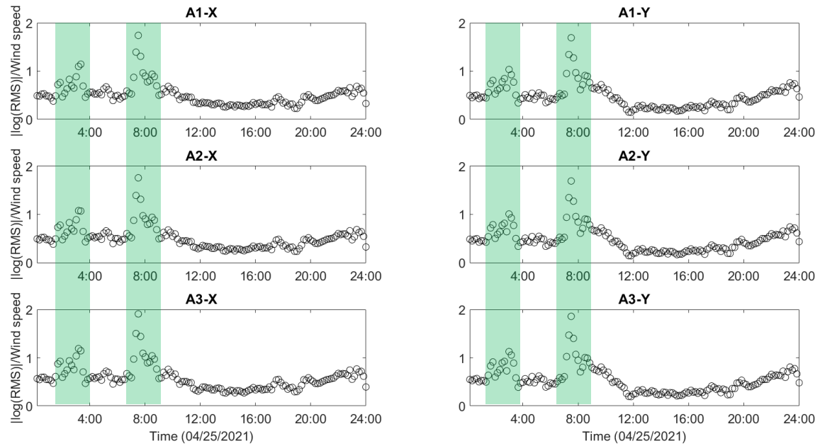
Figure 40. Evolution of |\log(RMS)|/\text{wind speed} (A1 – A3).
