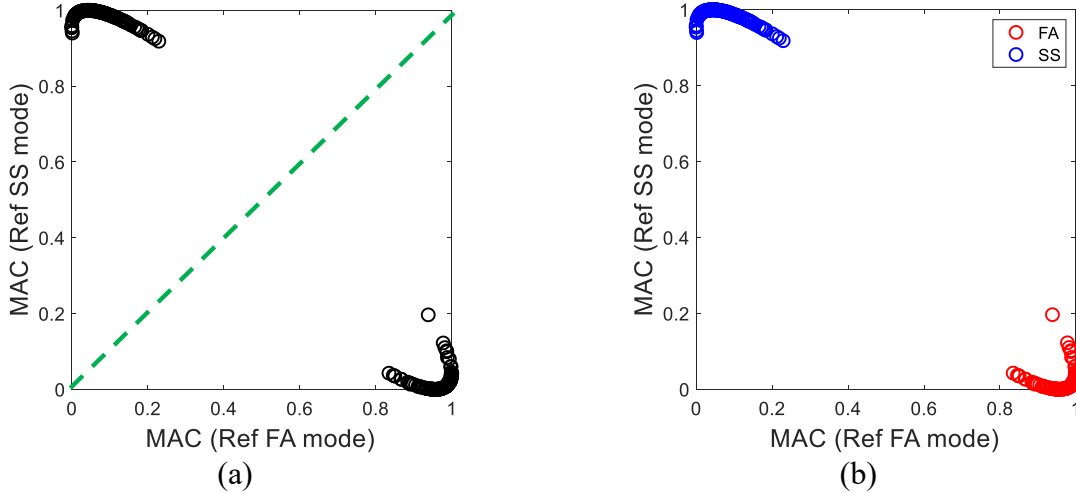
Figure 22. (a) MAC values with reference FA mode versus that with reference SS mode based on FA-SS coordinate; (b) FA/SS modes are well separated based on MAC values.
