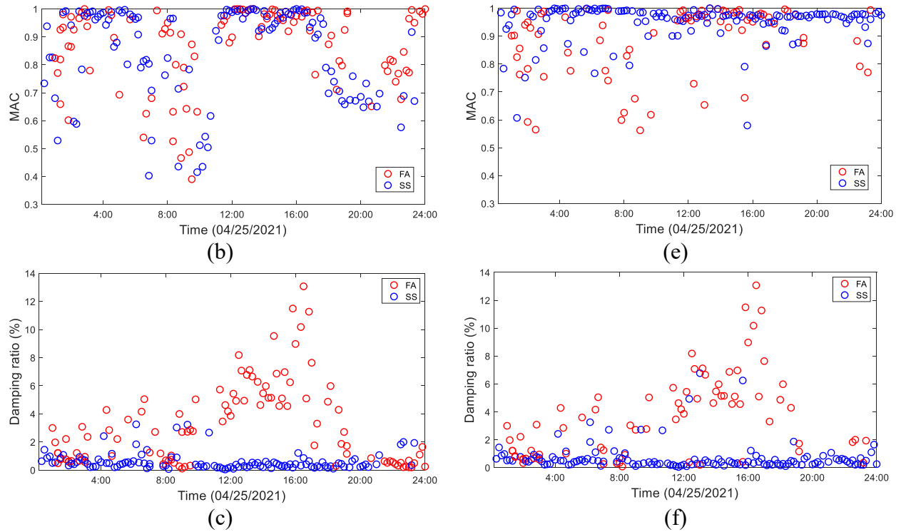
Figure 31. Frequencies, MAC and damping ratios evolution of identified FA/SS modes on April 25: (a – c) in global coordinate; (d – f) in FA-SS coordinate.
